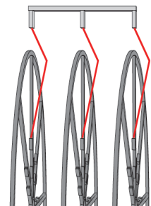
Figure 3: Inserting cross-braces.
